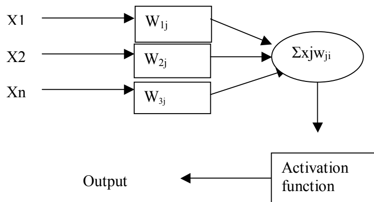
Figure 1 A Basic Neuron
